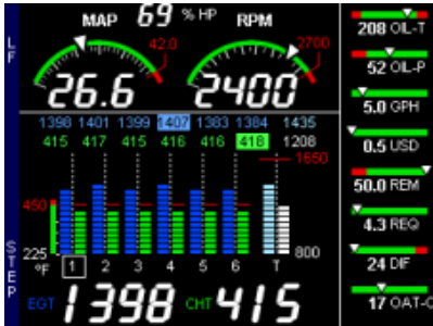
EDM-830 6 Cylinder (landscape orientation)
